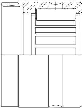
Single sealed cage type needle upper main bearing for outboard motor.
