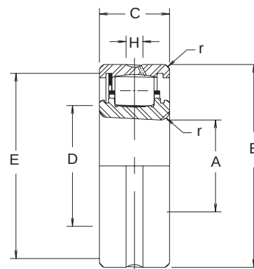
TAPERED BORE
