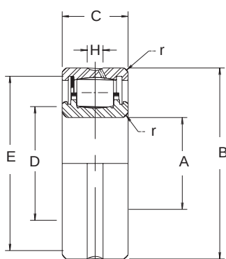
STRAIGHT BORE
